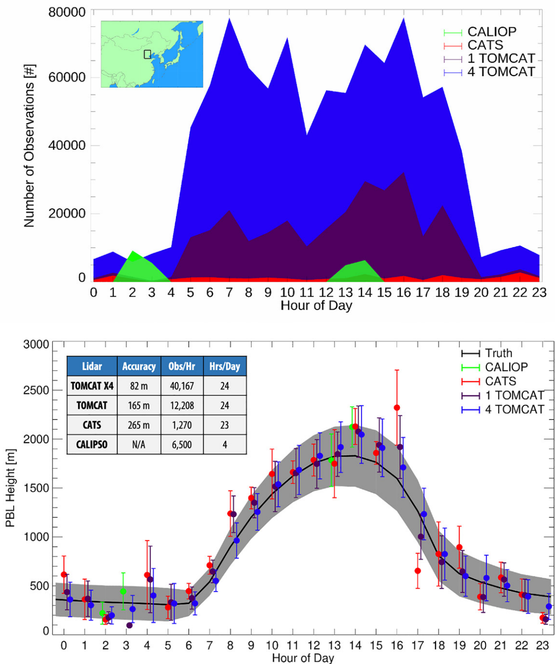
Fig. SB2. The TOMCAT mission concept provides data to statistically resolve the diurnal variability of PBLH on regional and seasonal scales. (top) For a 90-day period over a 5° latitude x 5° longitude grid box around Beijing, China (see inset), TOMCAT covers the entire diurnal cycle and provides more observations per hour than CATS and CALIPSO. (bottom) The TOMCAT spatiotemporal coverage also enables more accurate estimates of PBLH as a function of time of day.
